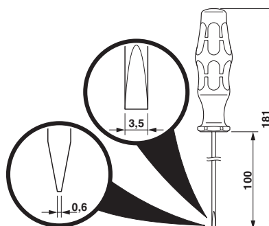
Dimensional drawing
